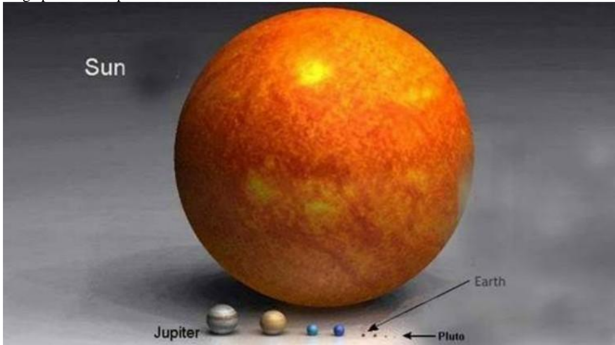
Large planets compared to the Sun:
