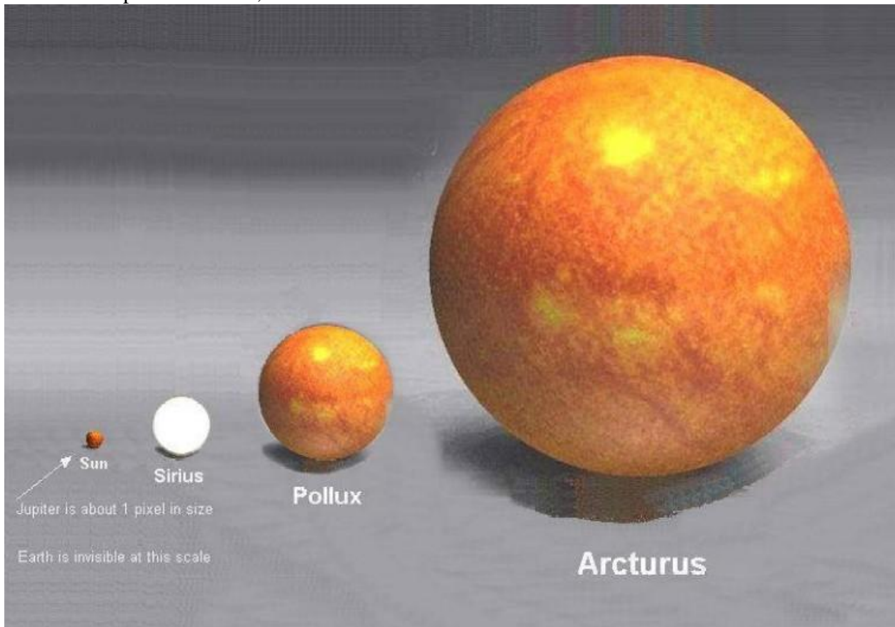
Our Sun compared to Sirius, Pollux and Arcturus:
